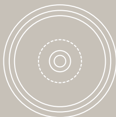
HASU 44 - art. HS44A lavabo appoggio/su colonna countertop/on pedestal basin cm Ø 44 x 18
