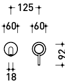
vista frontale / frontal view
