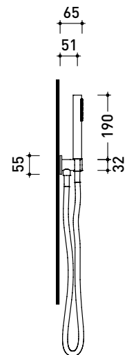
vista laterale / lateral view
