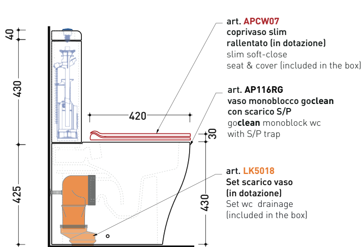
vista laterale / lateral view
