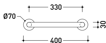
vista frontale / frontal view
