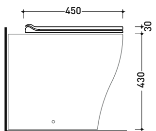
art. AP117G - AP117RG vista laterale / lateral view
