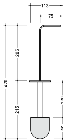
scopino / toilet brush
