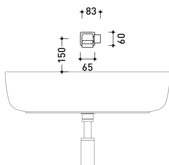
vista frontale / frontal view
