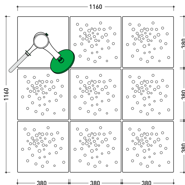
vista zenitale / zenital view 8pcs art. ABM + art. AB238
