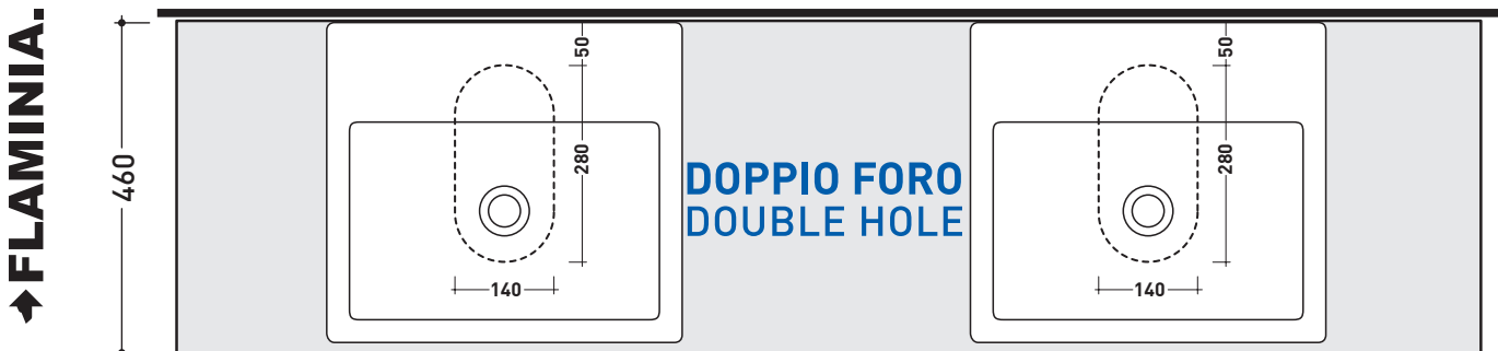
lavabo / basin 5058 - FG64L - FU60L - FU70L
