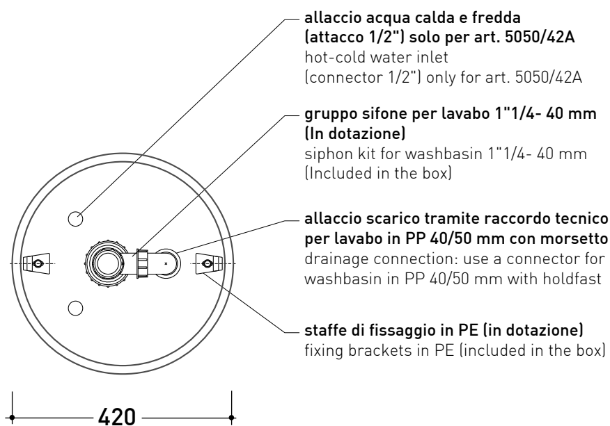
pianta attacco a terra / floor fixing plan
